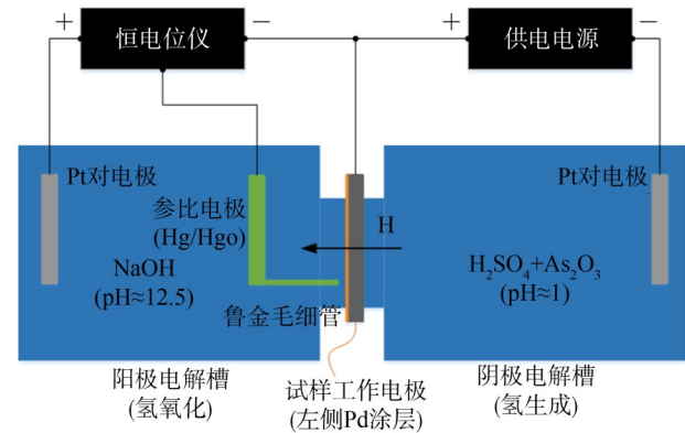
图 1 D-S 双电解槽电化学氢渗透试验测氢原理示意 Fig. 1 Schematic diagram of hydrogen measurement principle in D-S double electrolytic cell electrochemical hydrogen permeation test
