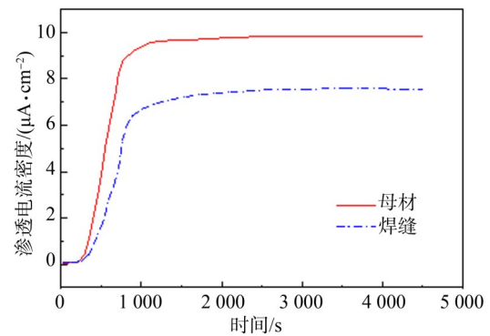
图 2 Ti6Al4V 的母材和焊缝的氢渗透曲线 Fig. 2 Hydrogen permeation curves of weld seam and base metal of Ti6Al4V alloy
